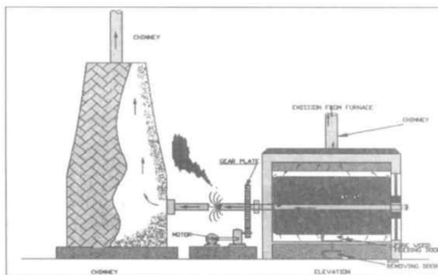
Flow diagram of Calcination process and emissions source
